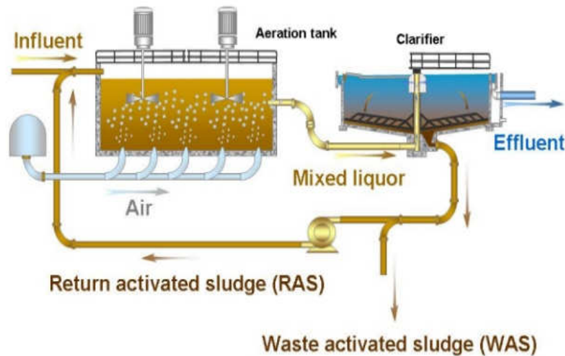
Gambar 34 Skema Extended Aeration
