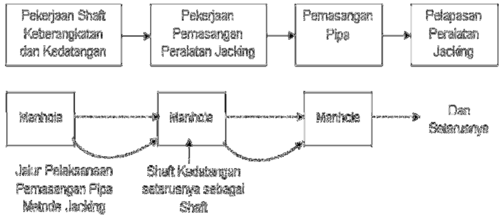
Gambar 41 Tahap Pelaksanaan Metode microtunneling/jacking
